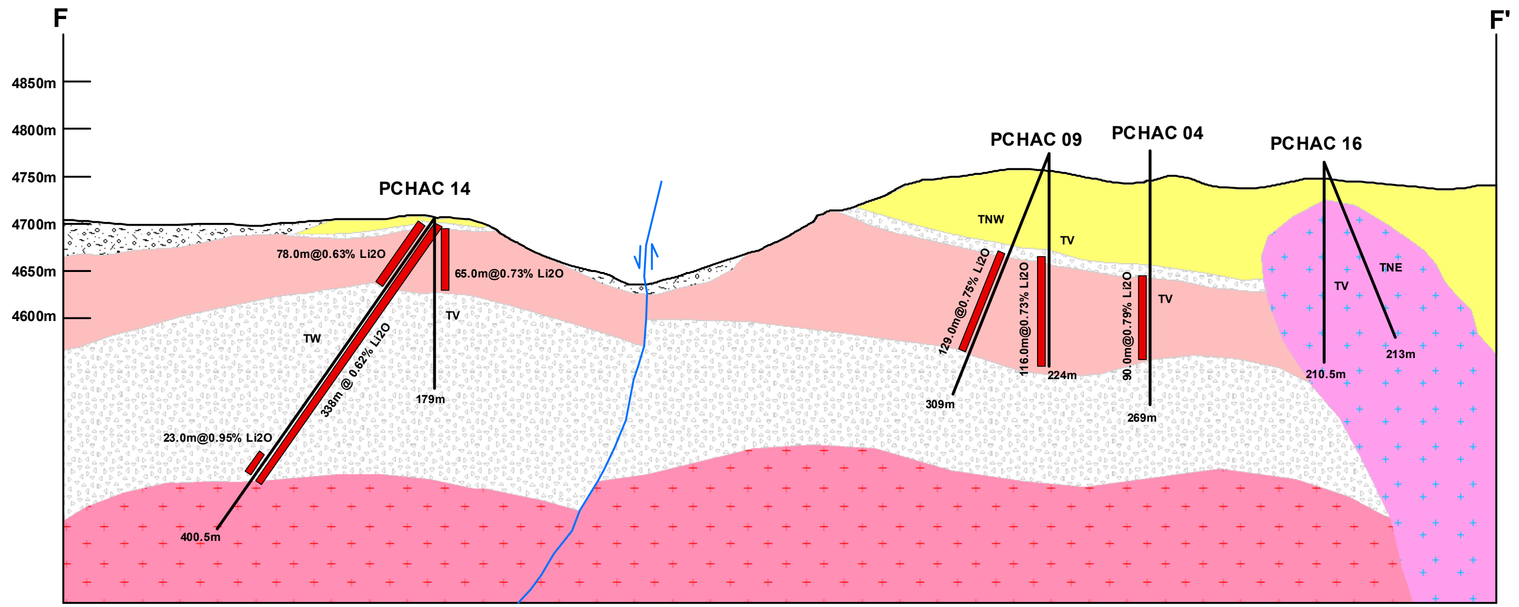
F - F' CROSS SECTION LOOKING NORTH THROUGH FALCHANI WEST TO EAST ZONES
