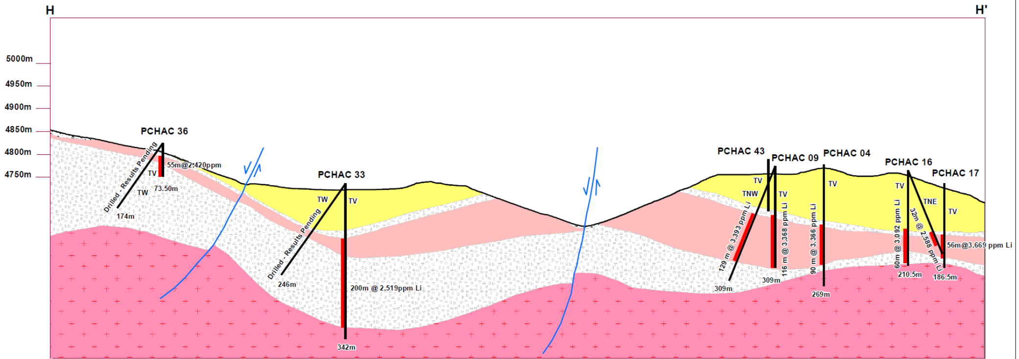
H- H' CROSS SECTION LOOKING NORTH THROUGH FALCHANI WEST TO EAST ZONES
